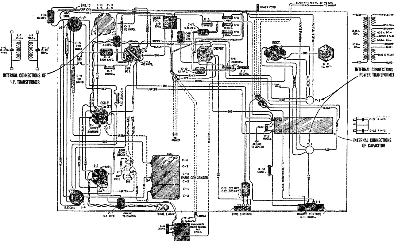
Figure D—Wiring Diagram
